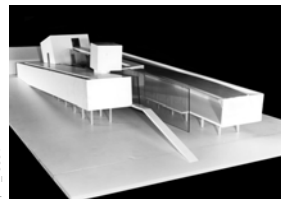
1990 NEW OFFICE BUILDING OPTIMUM DATA Baden Austria A multifunctional office building
